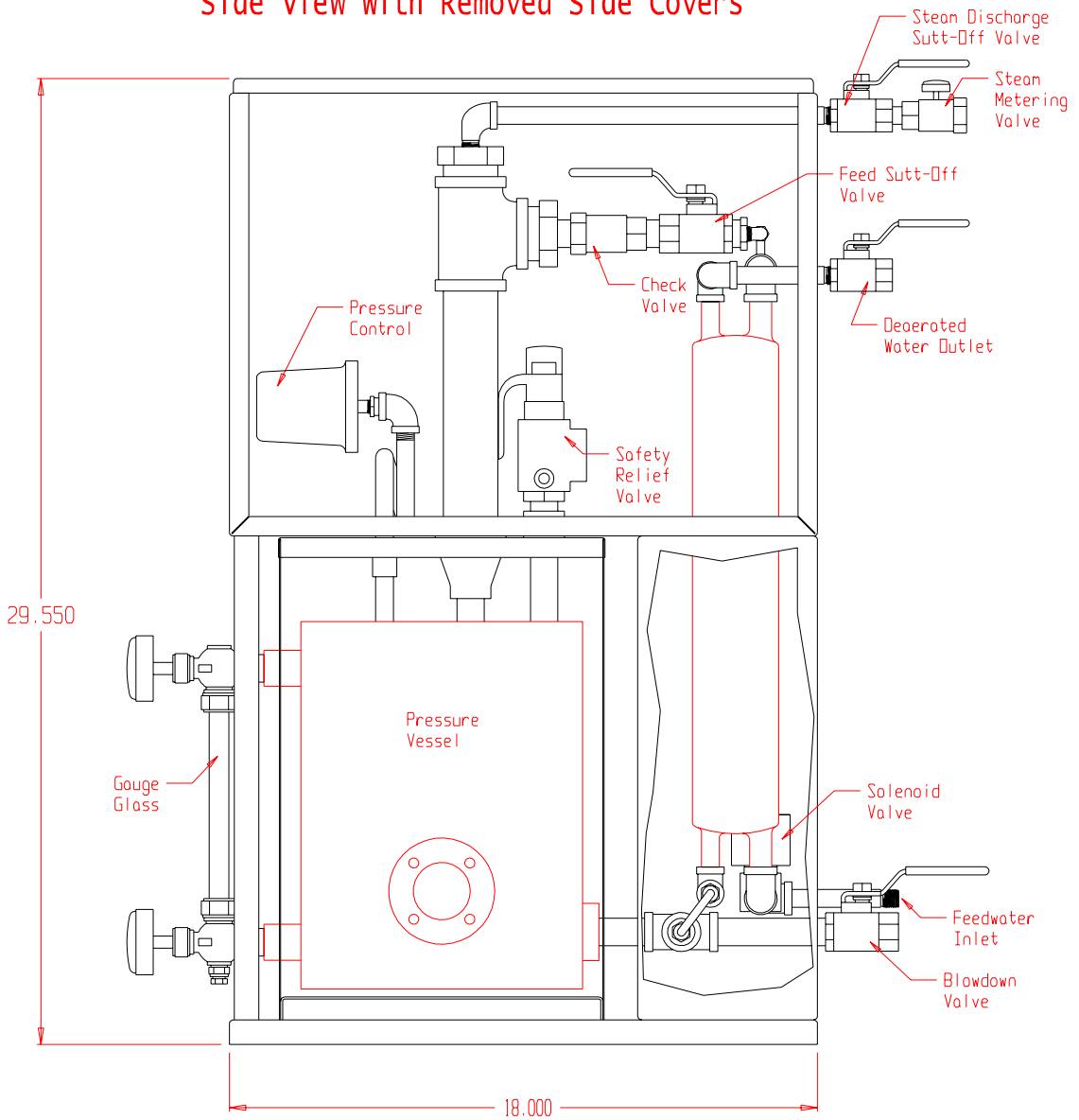
Side view with Removed Side Covers
